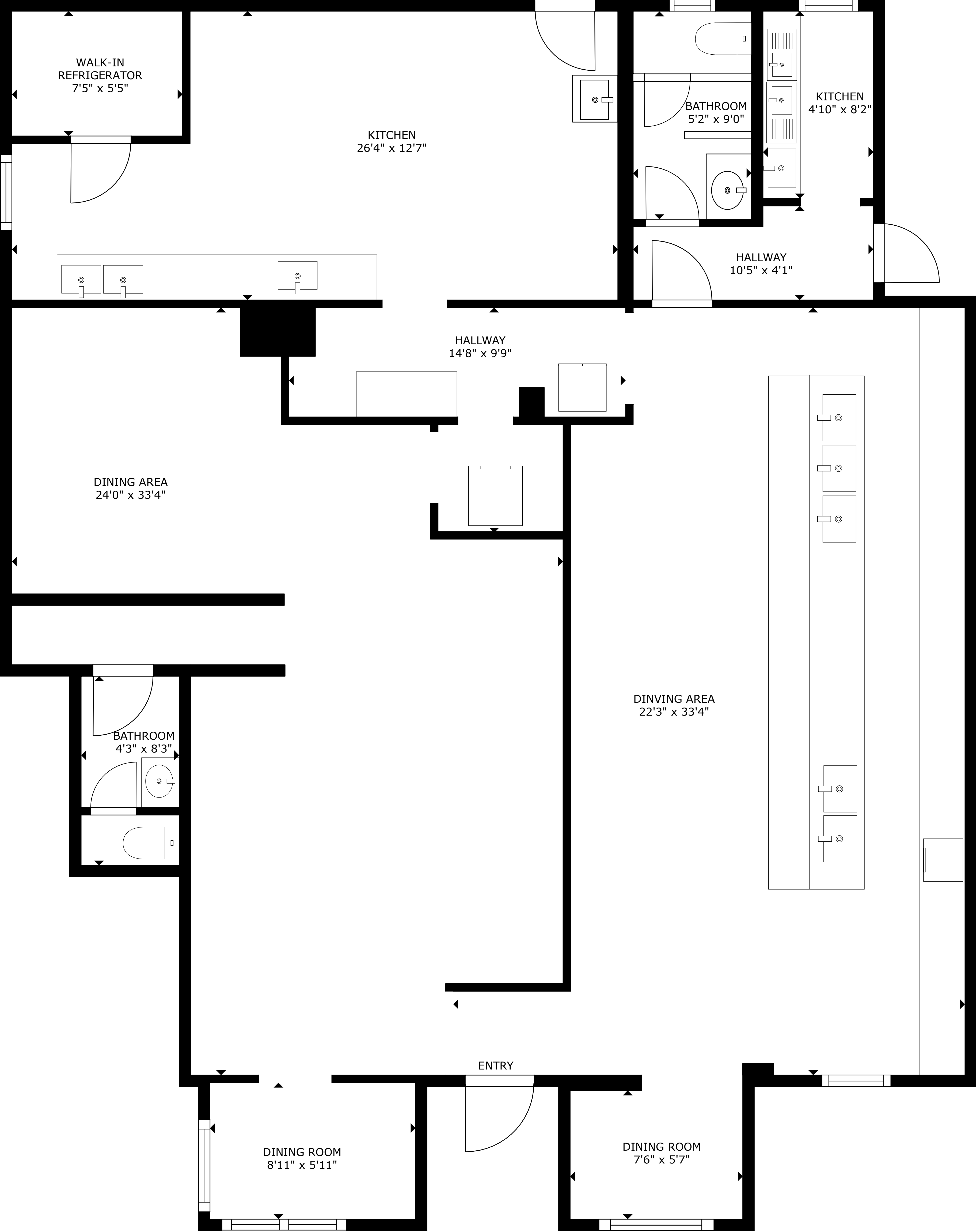
FLOOR PLAN
